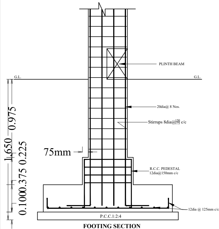
FOOTING SECTION
