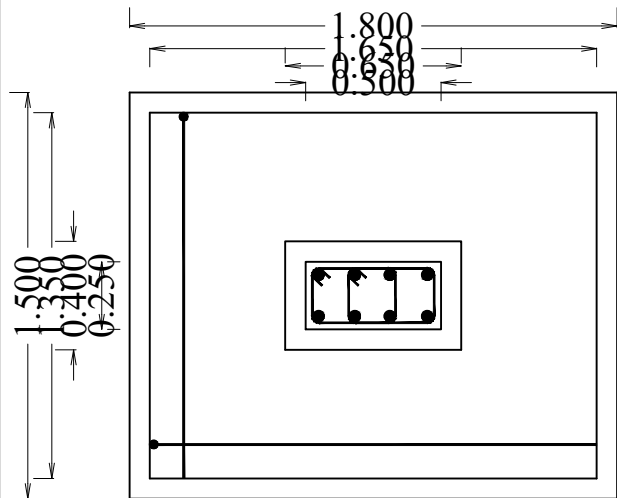
FOOTING PLAN
