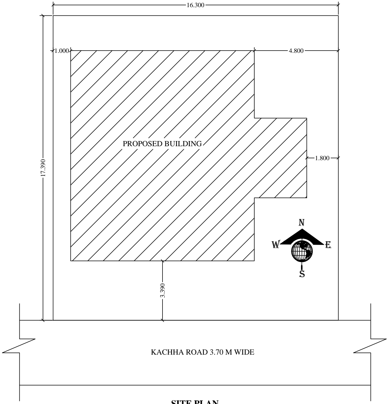
SITE PLAN
