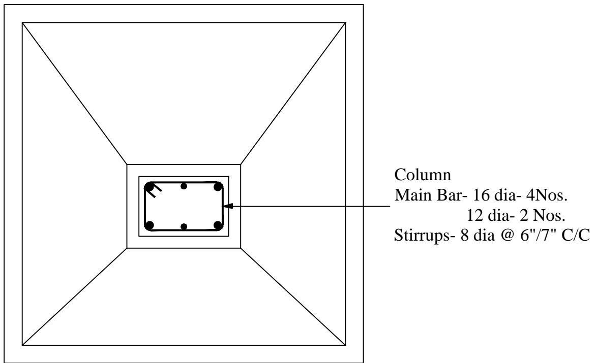
FOOTING PLAN & SECTION
