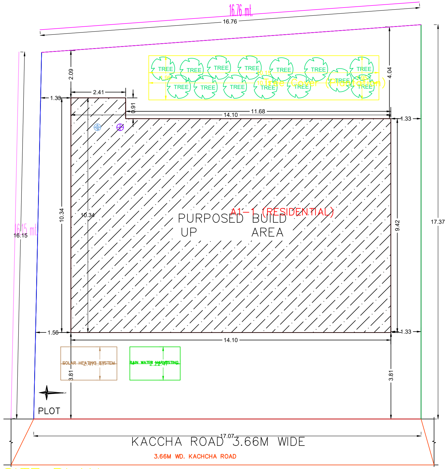
SITE PLAN
