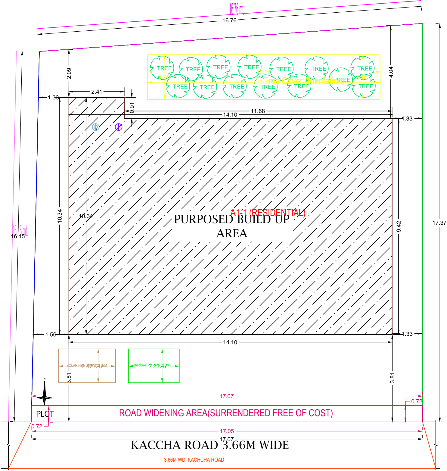
SITE PLAN
