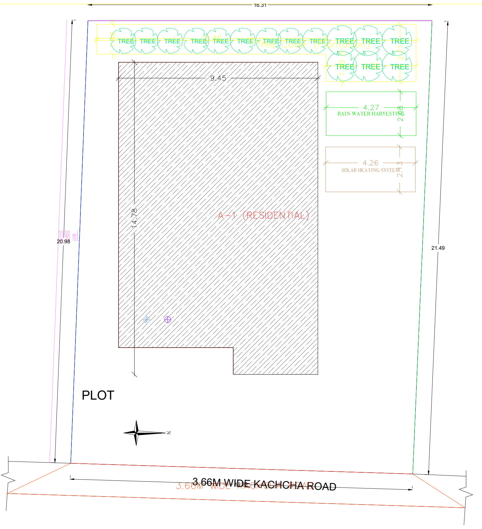
SITE PLAN
