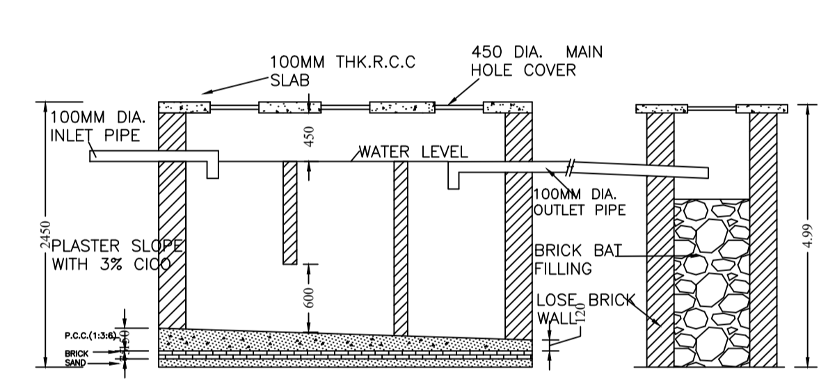
SECTION-DD
