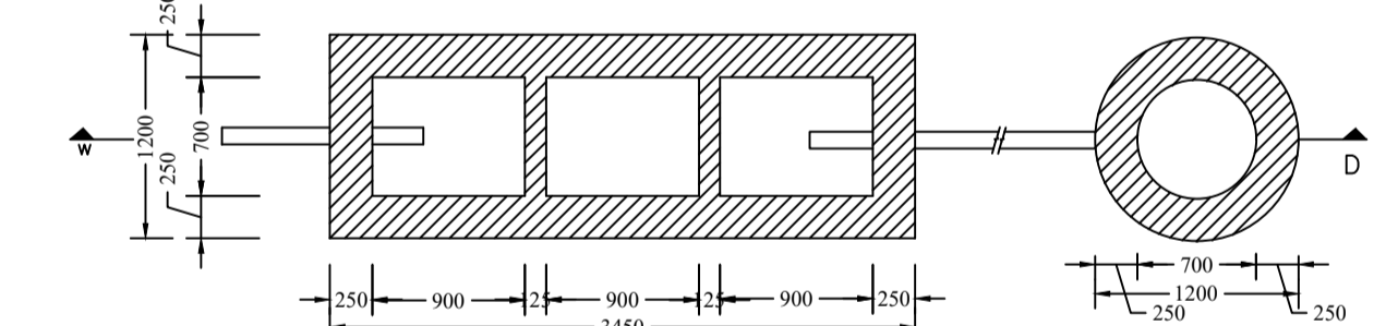
DETAIL OF SEPTIC TANK & SOAKPIT (SCALE 1:50)
