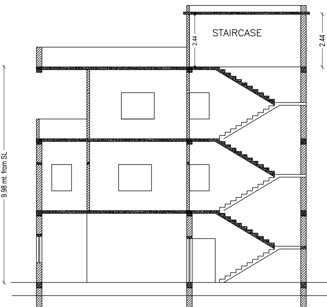
SECTION ON (SCALE 1:100)
