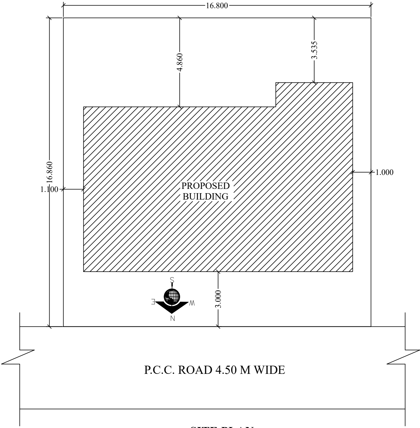
SITE PLAN
