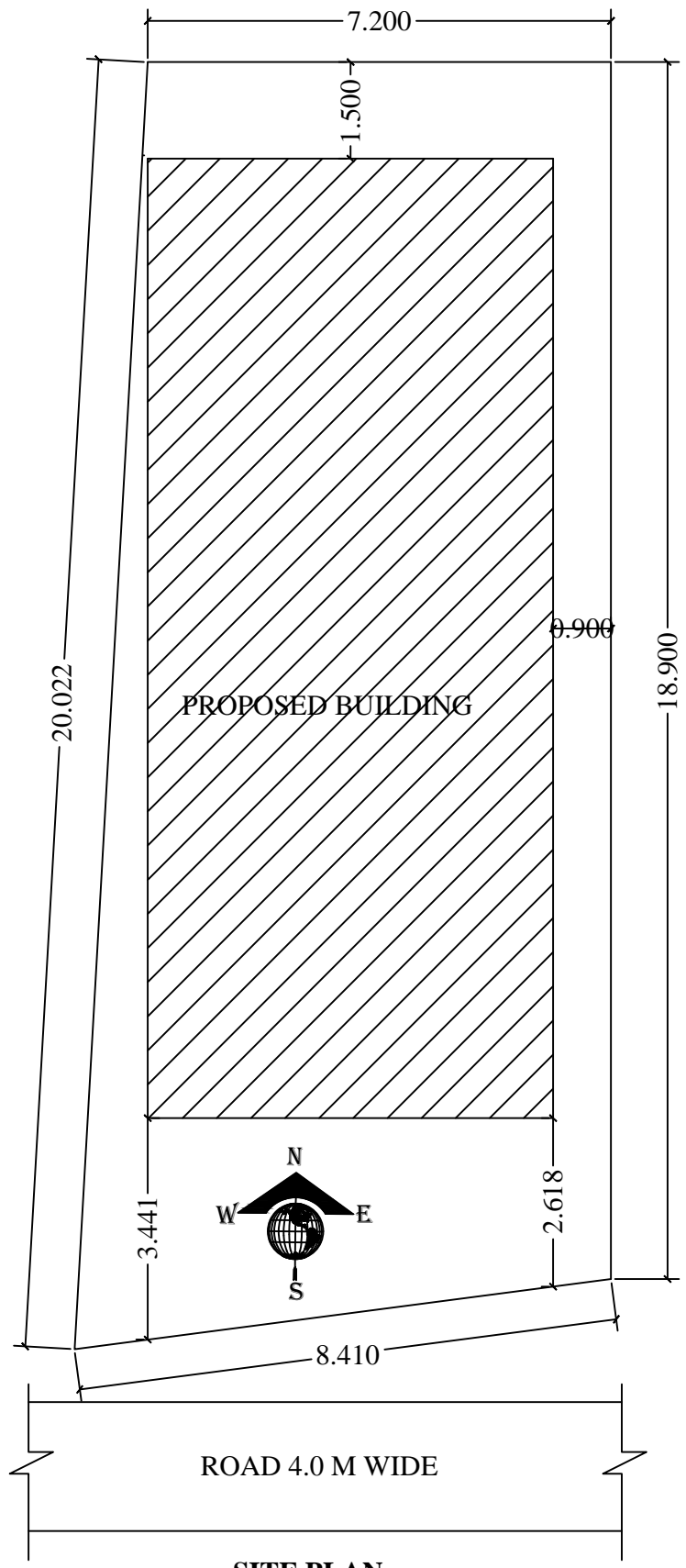
SITE PLAN
