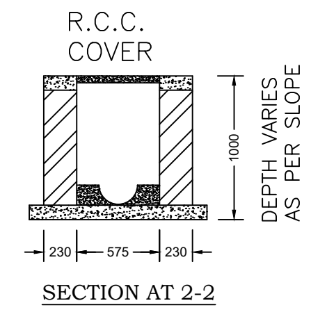
PLAN I.C. DETAILS R.C.C. COVER (SECTION AT 2-2)
