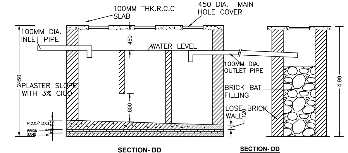
SECTION-DD
