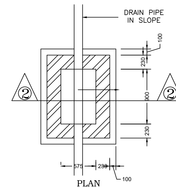
PLAN I.C. DETAILS R.C.C. COVER (SECTION AT 2-2)
