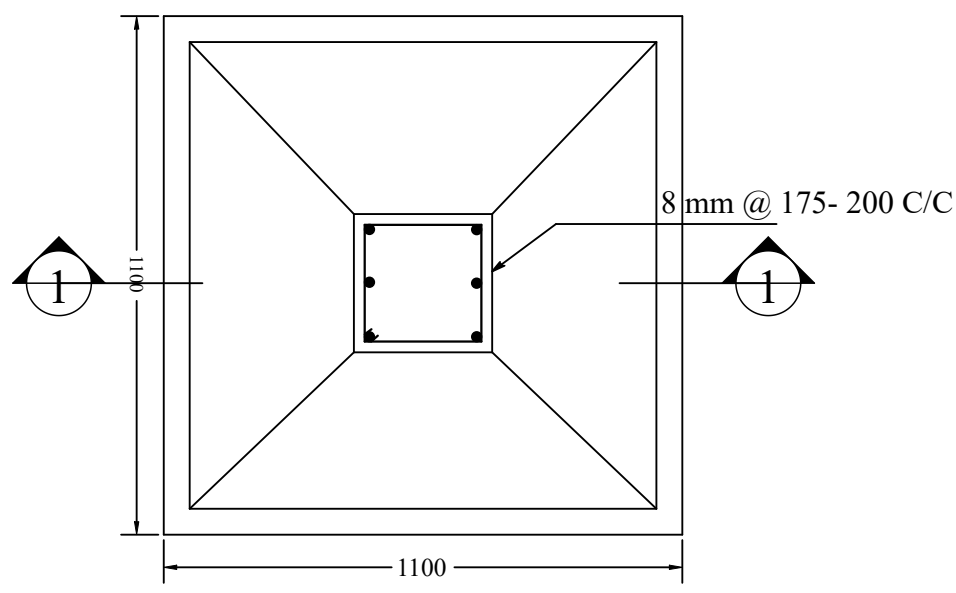
6 Nos.- 12 mm Dia Bar TYPICAL FOUNDATION SCALE -1:25
