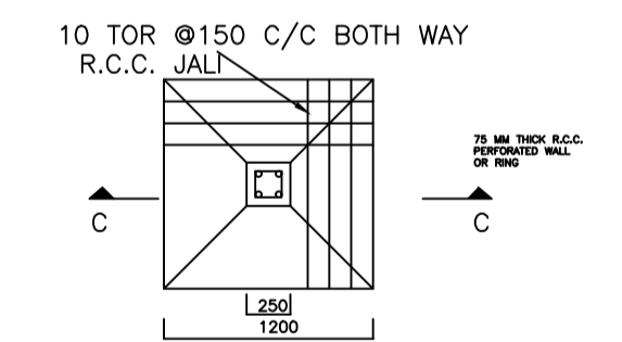
DETAIL OF FOUNDATION
