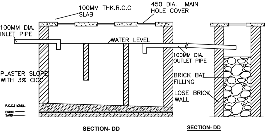
SECTION-DD
