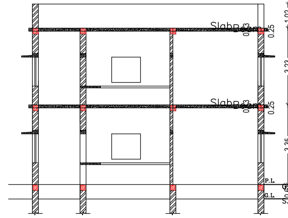
SECTION ON SCALE 1:100
