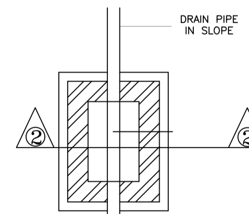
DETAIL OF SEPTIC TANK & SOAKPIT.
