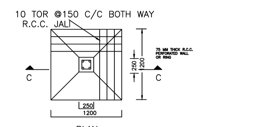
DETAIL OF FOUNDATION (SCALE: 1:5)
