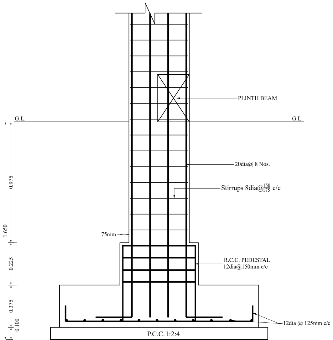
FOOTING SECTION
