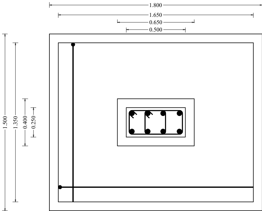
FOOTING PLAN
