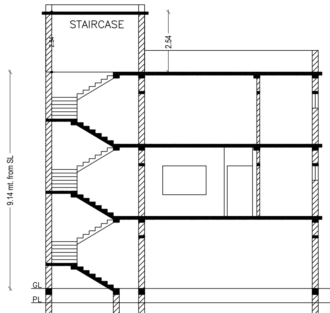
SECTION ON SCALE 1:100
