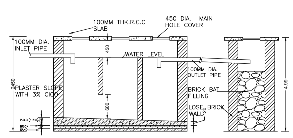
SECTION-DD
