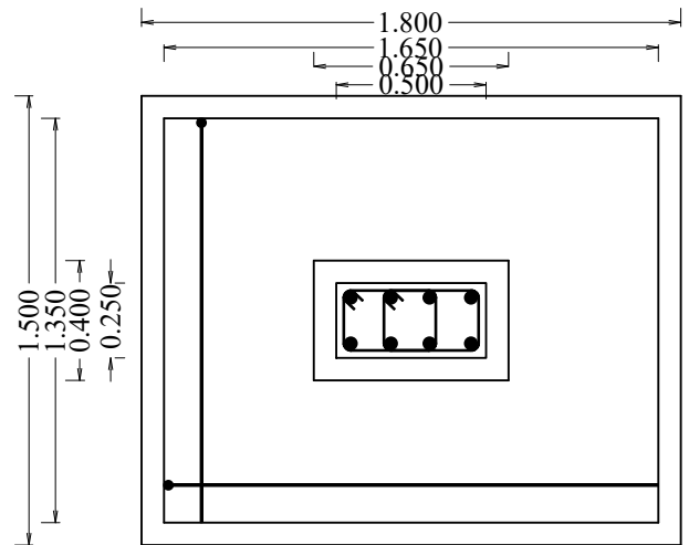
FOOTING PLAN
