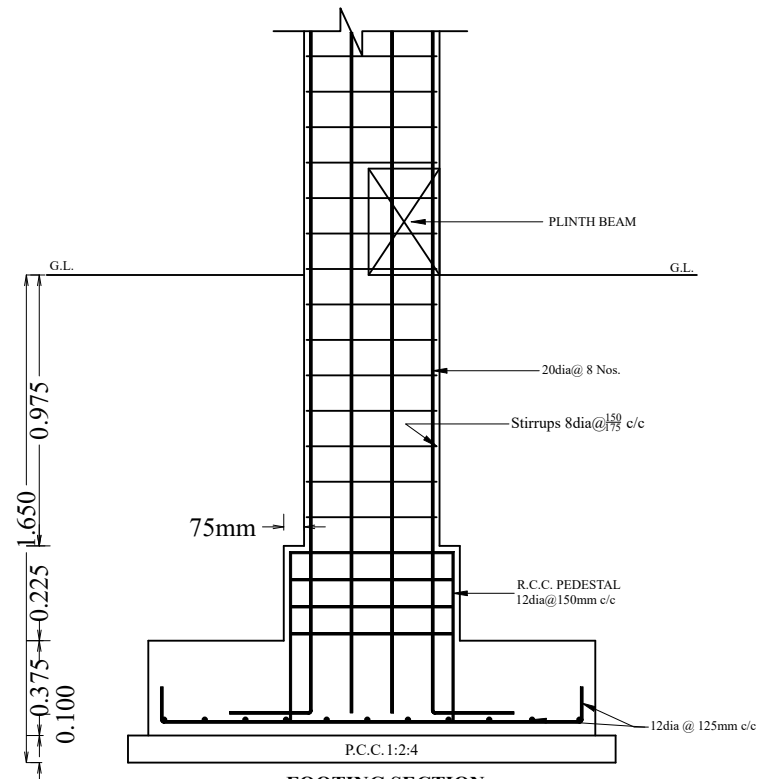
FOOTING SECTION
