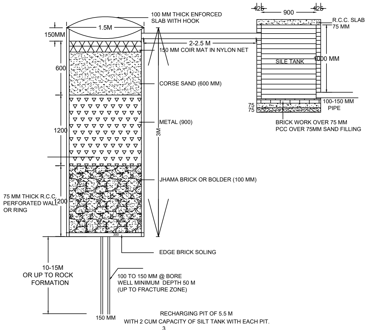
RECHARGING PIT OF 5.5 M WITH 2 CUM CAPACITY OF SILT TANK WITH EACH PIT. 3 DESIGN OF RECHARGE PIT FOR ROOF TOP RAIN WATER HARVESTING
