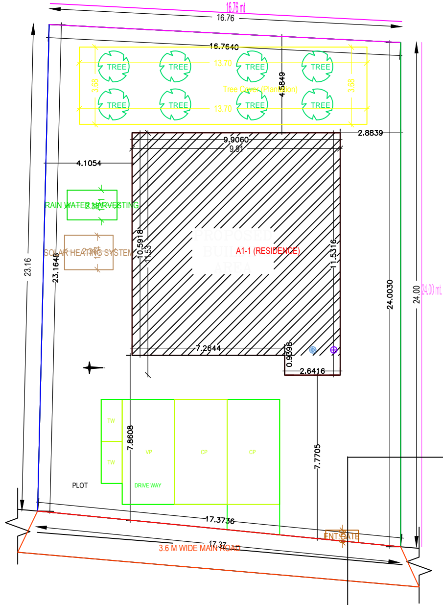
SITE PLAN
