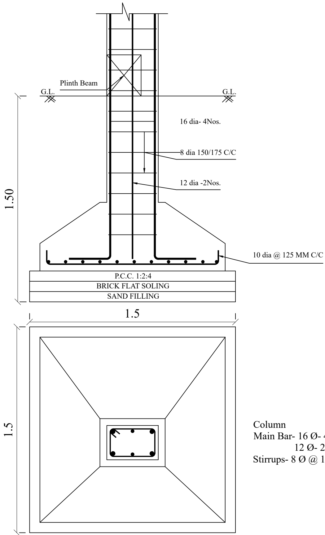
FOOTING PLAN & SECTION
