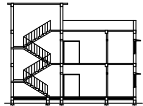
SECTION AT X-X
