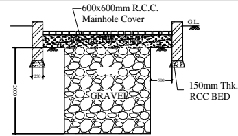
SECTION '3-3'
