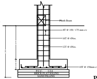
SECTION
