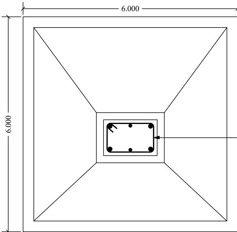
FOOTING PLAN & SECTION
