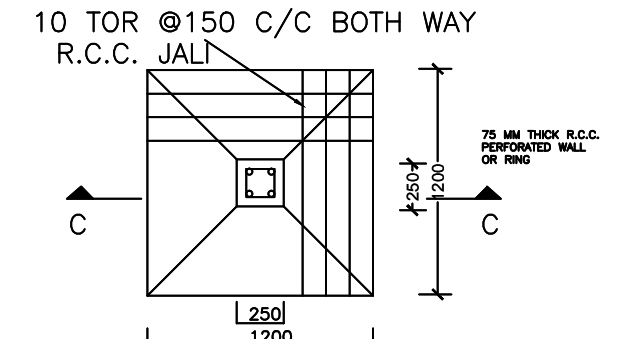
PLAN OF FOUNDATION
