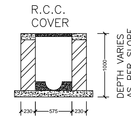
SECTION AT 2-2
