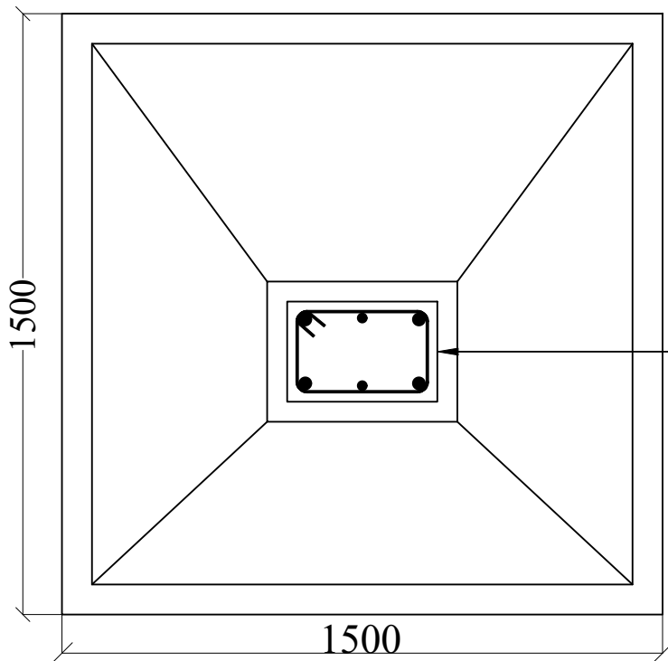
FOOTING PLAN & SECTION
