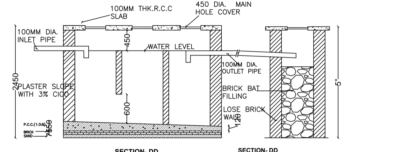
SECTION-DD
