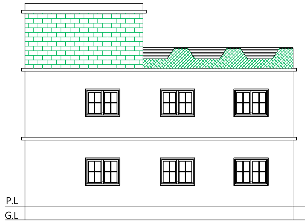
RIGHT ELEVATION SCALE 1:100
