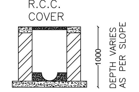
SECTION AT 2-2
