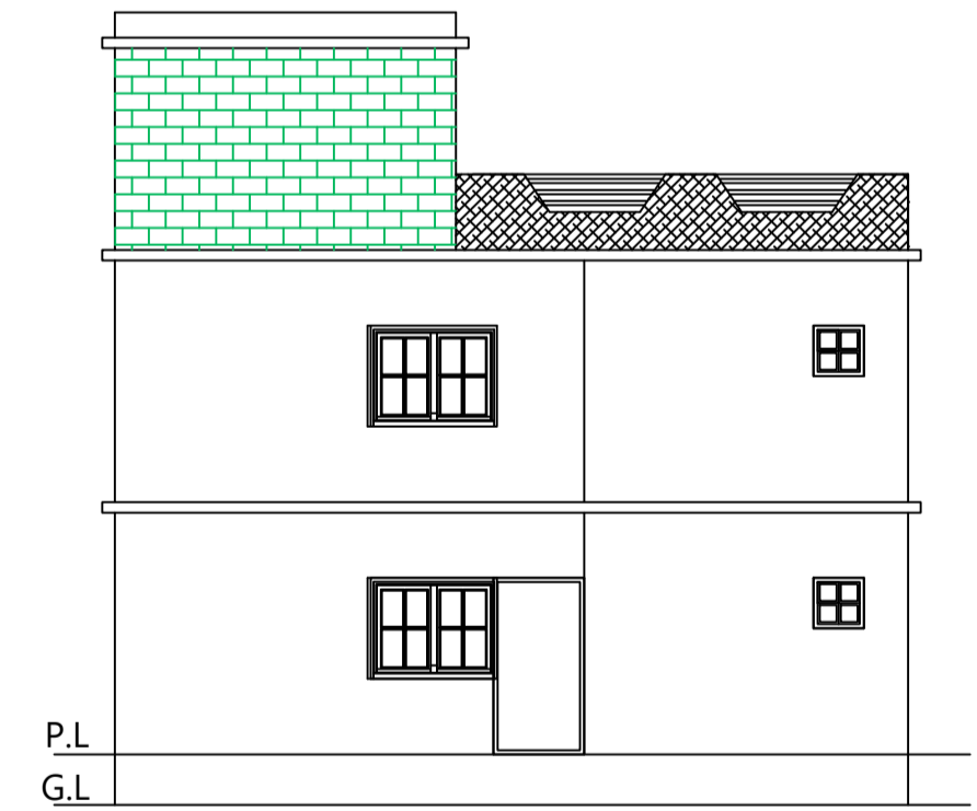
FRONT SIDE ELEVATION SCALE 1:100
