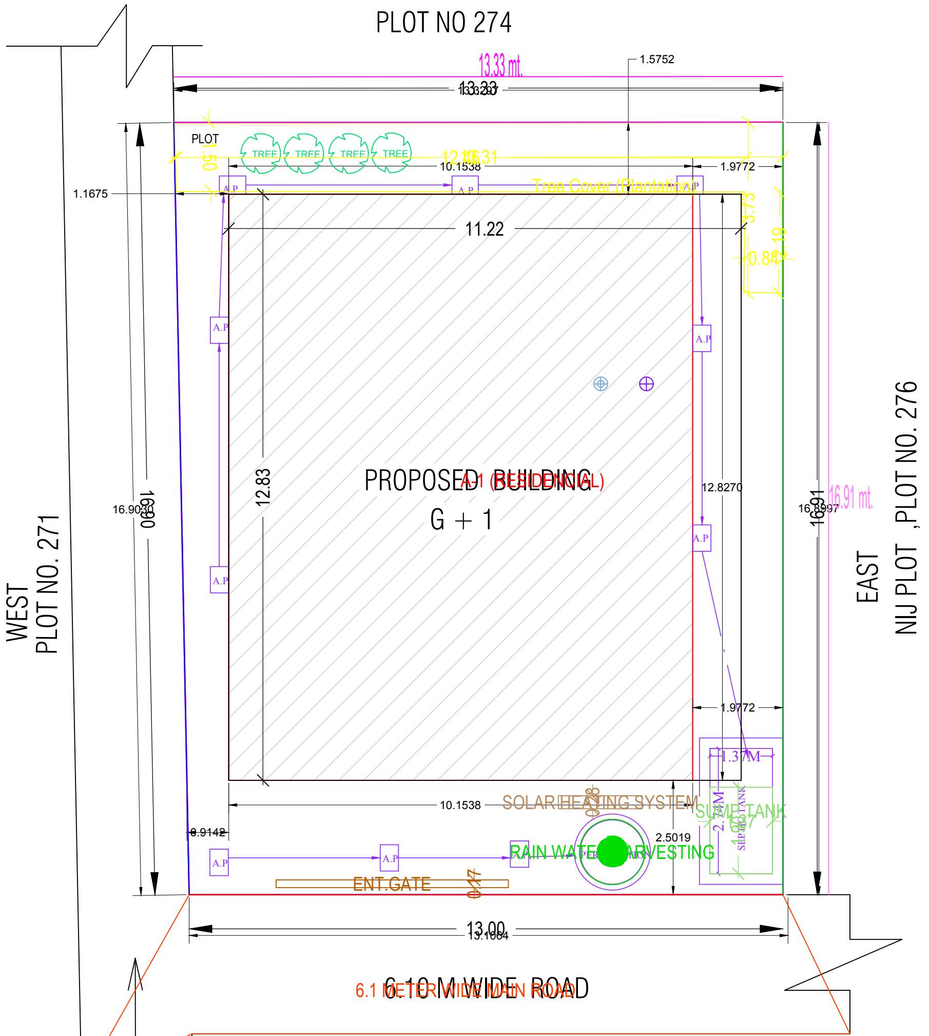
KEY PLAN SCALE - 1:200
