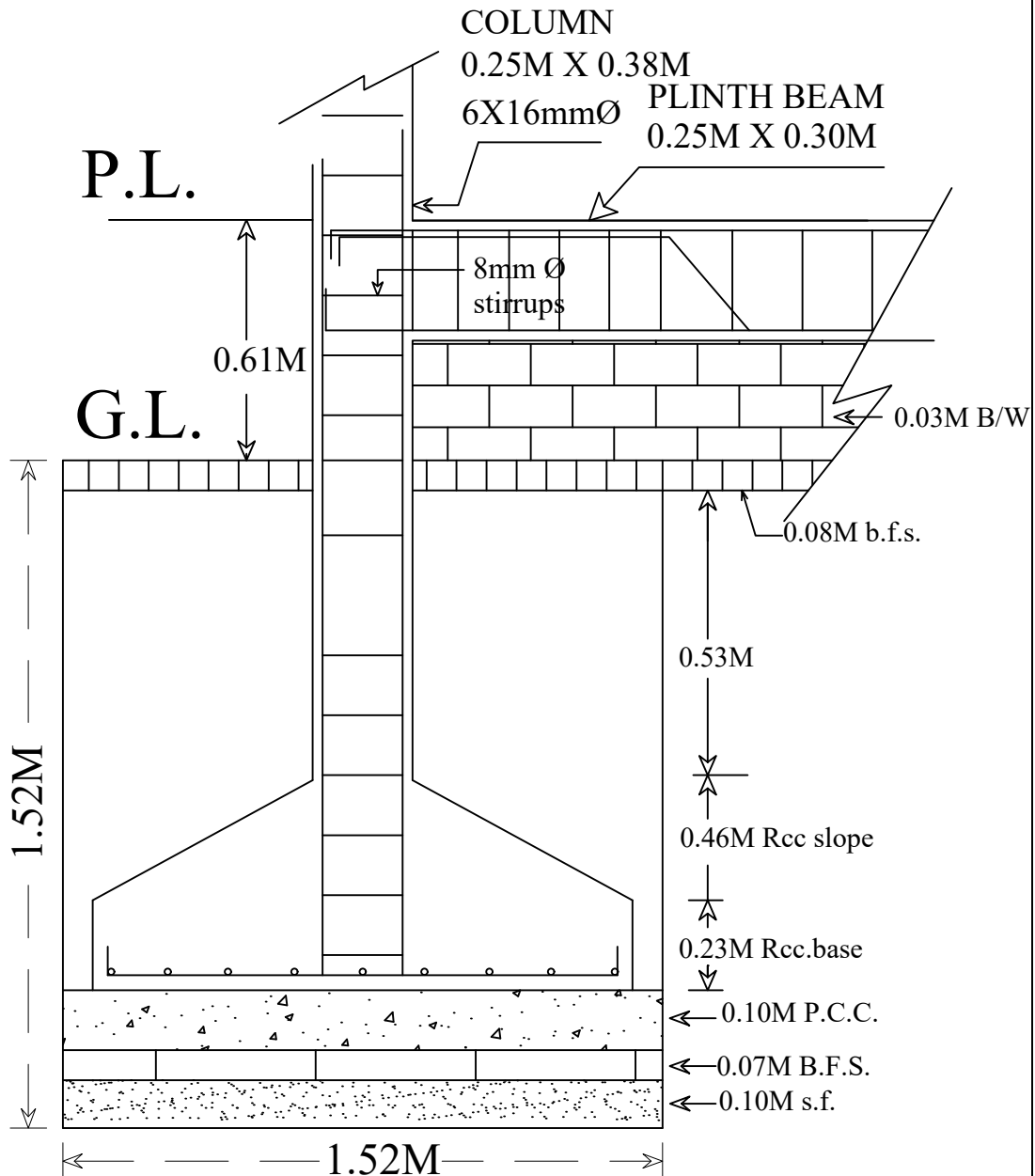
Structure Detail C/S OF FOOTING
