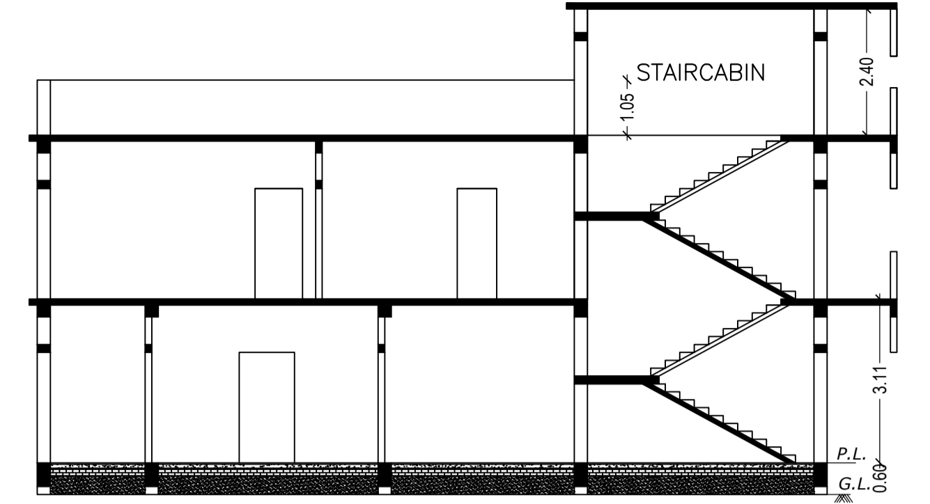
C/S AT X-X'
