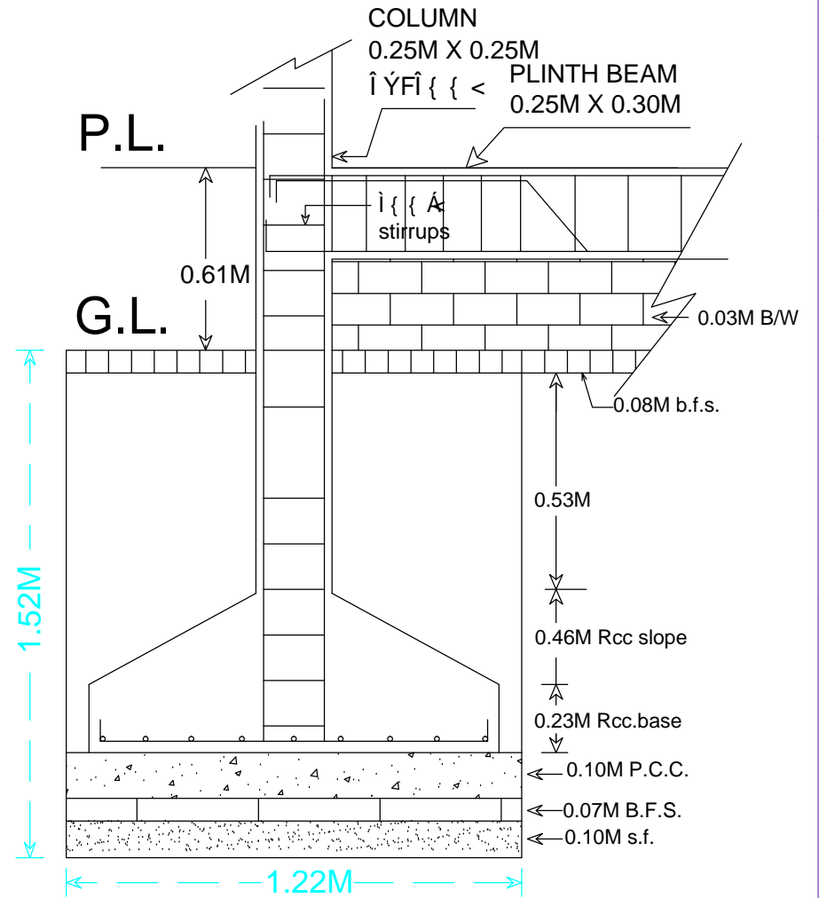
C/S OF FOOTING
