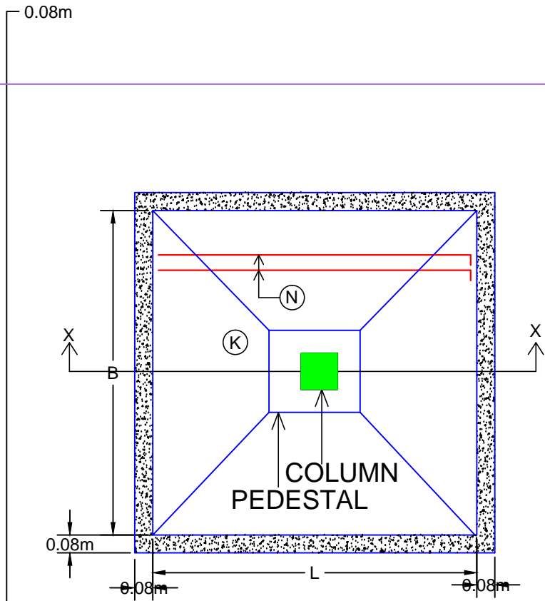
PLAN OF ISOLATED FOOTING
