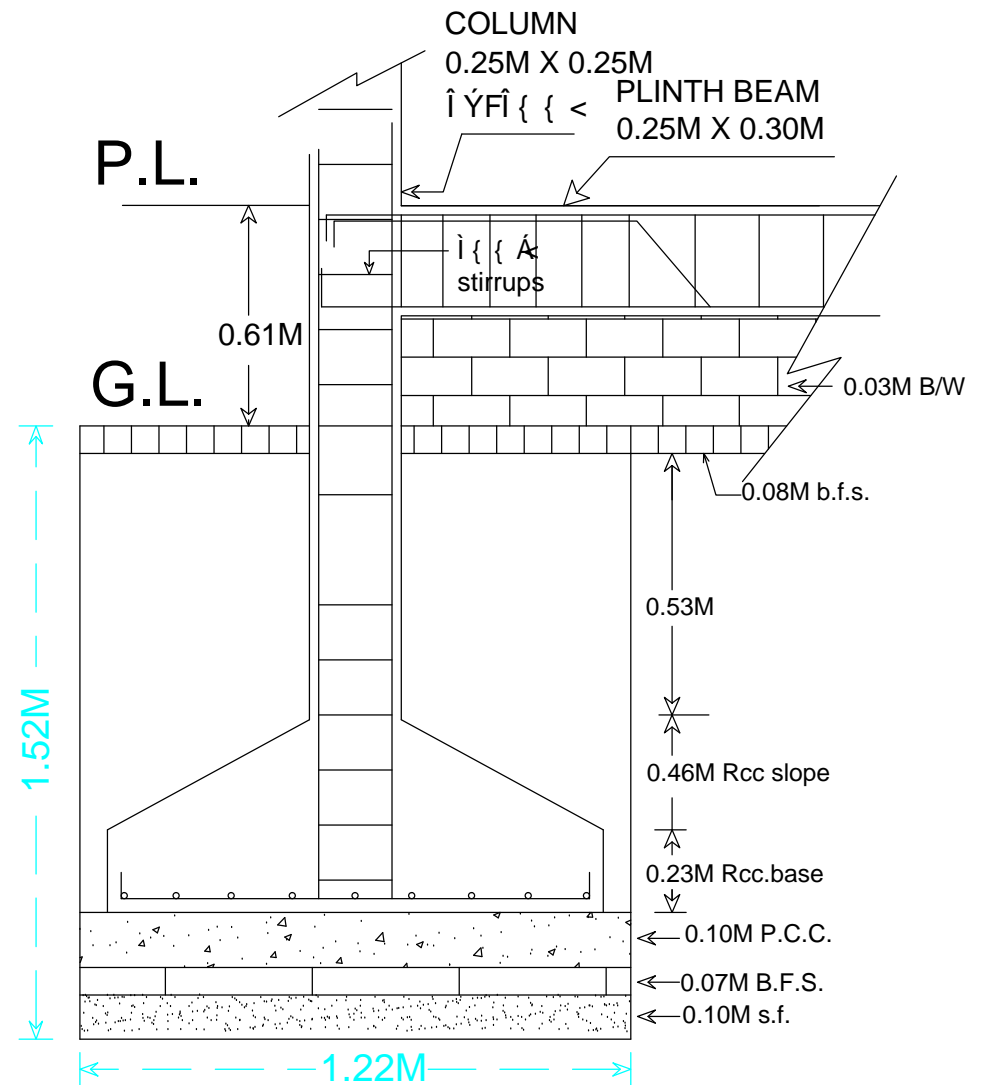
C/S OF FOOTING
