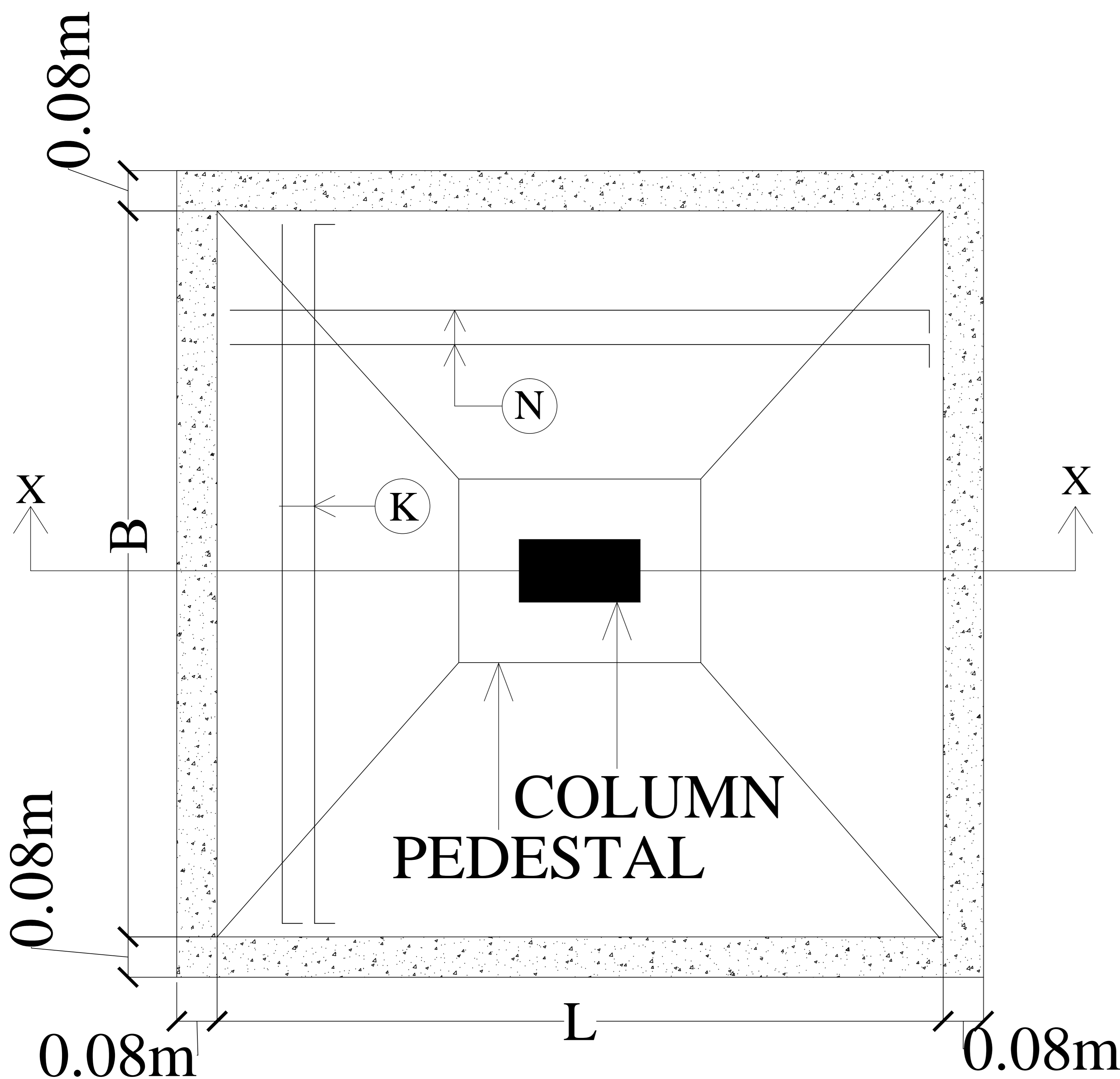
PLAN OF ISOLATED FOOTING
