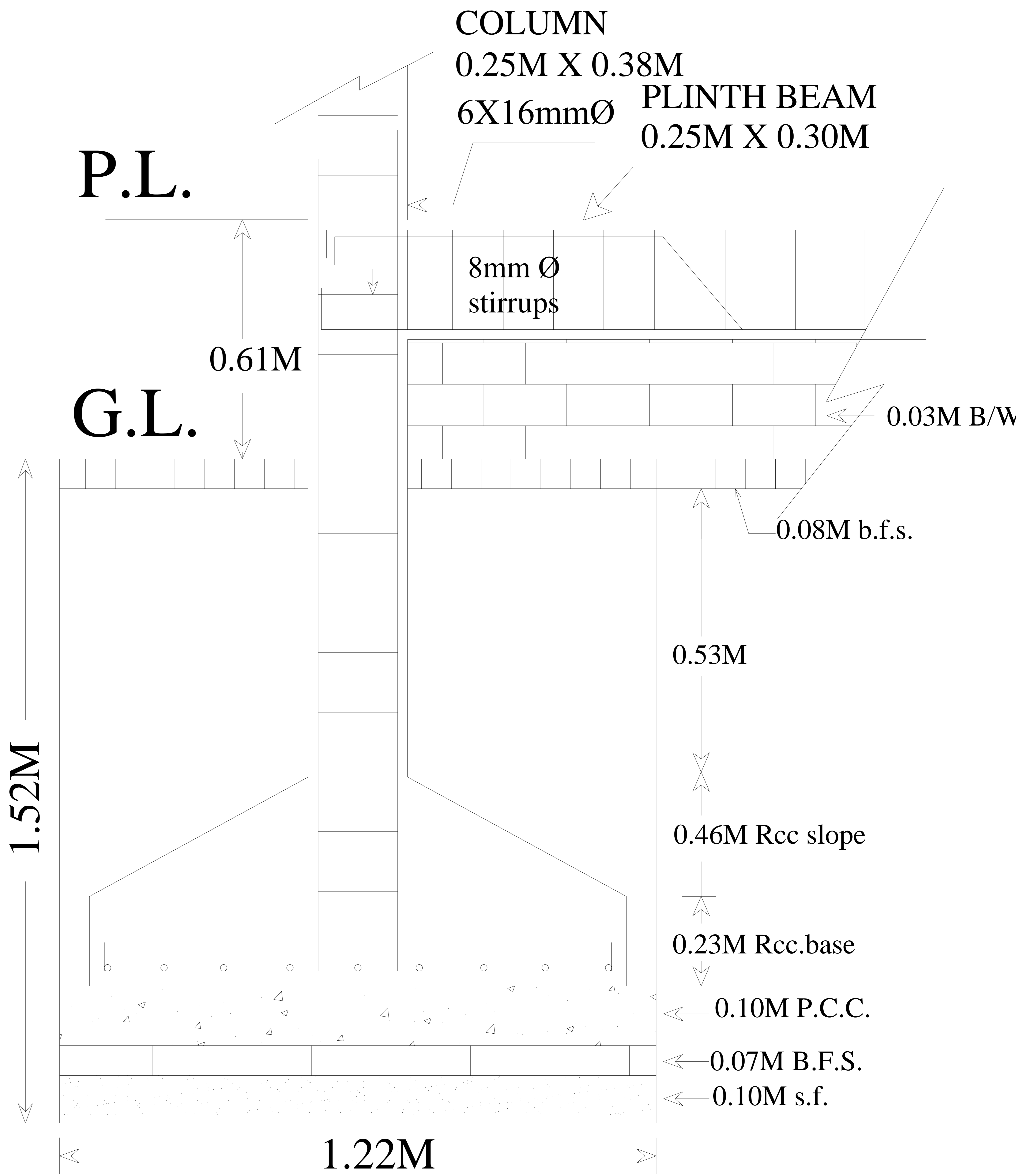
C/S OF FOOTING
