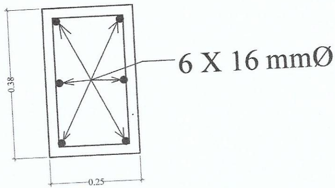
SECTION OF COLUMN.
