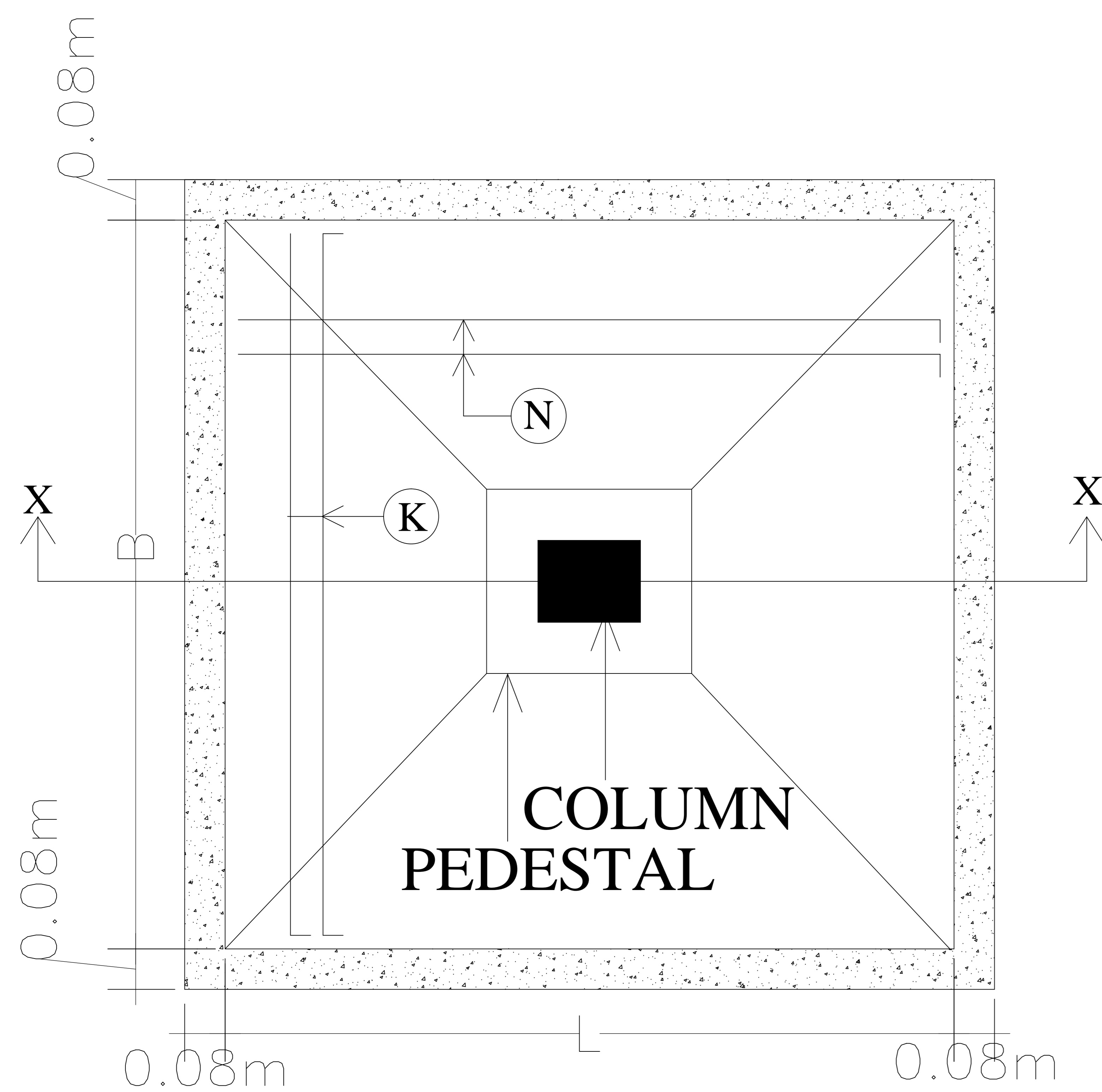
PLAN OF ISOLATED FOOTING
