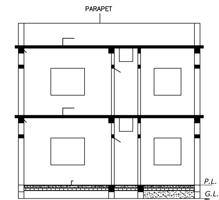
C/S AT A-A'
