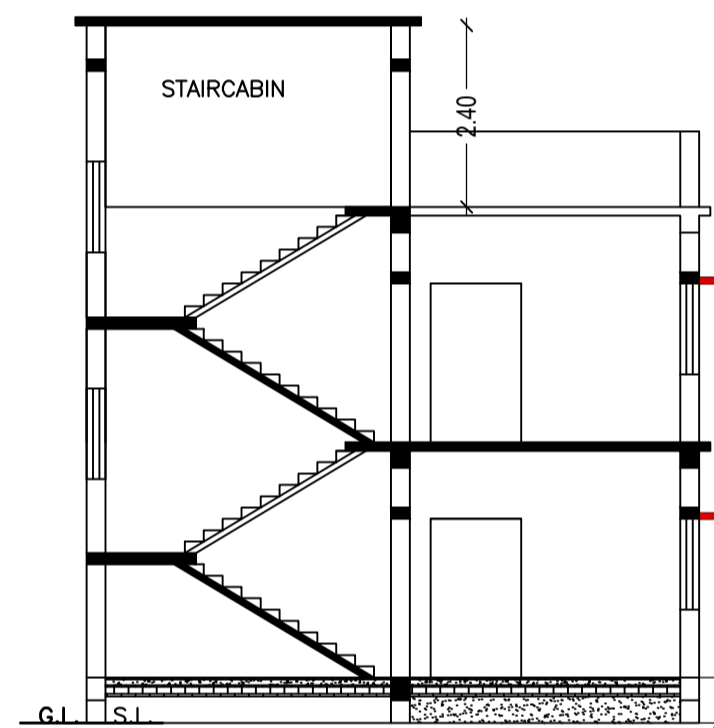
C/S AT X-X'
