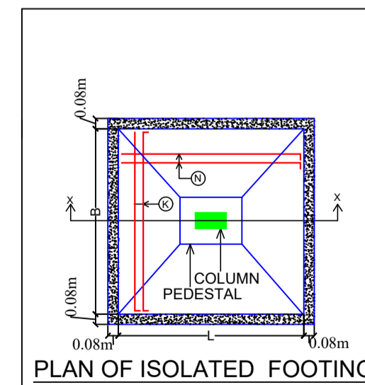
PLAN OF ISOLATED FOOTING
