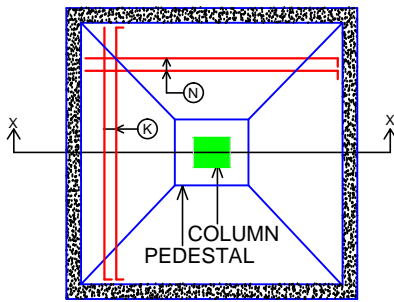
PLAN OF ISOLATED FOOTING
