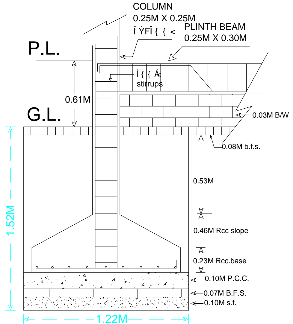
C/S OF FOOTING
