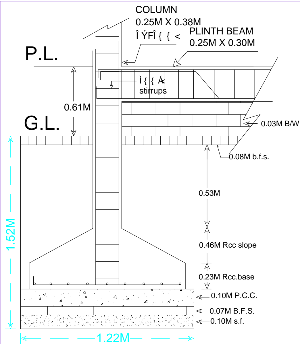
Structure Detail OF FOOTING
