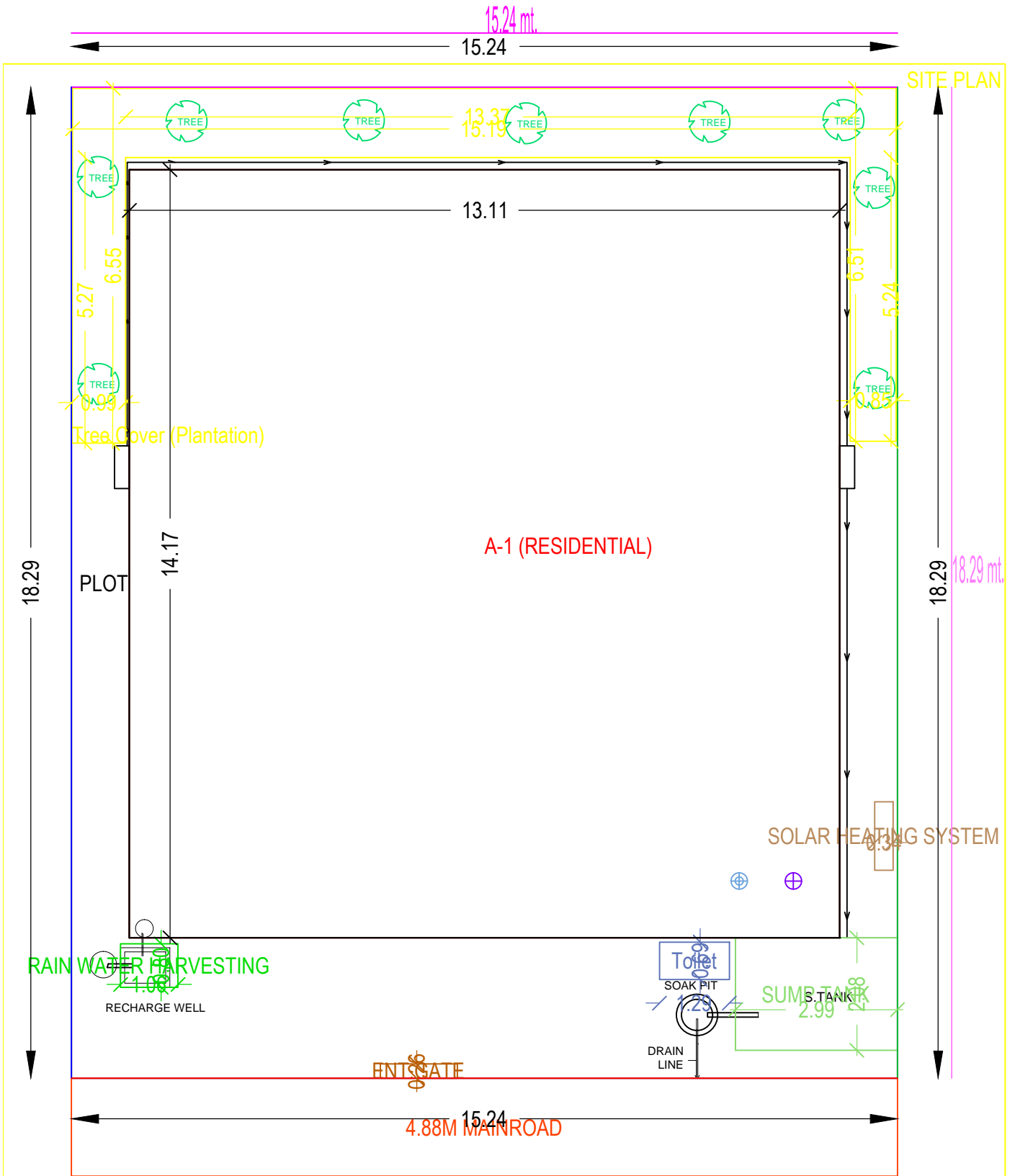
NORTH SIDE ROAD & FRONT SCALE: 1:100
