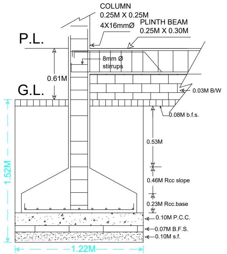
C/S OF FOOTING
