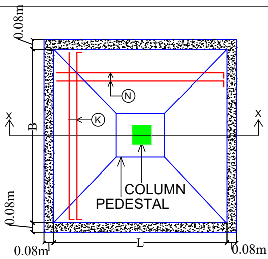
PLAN OF ISOLATED FOOTING
