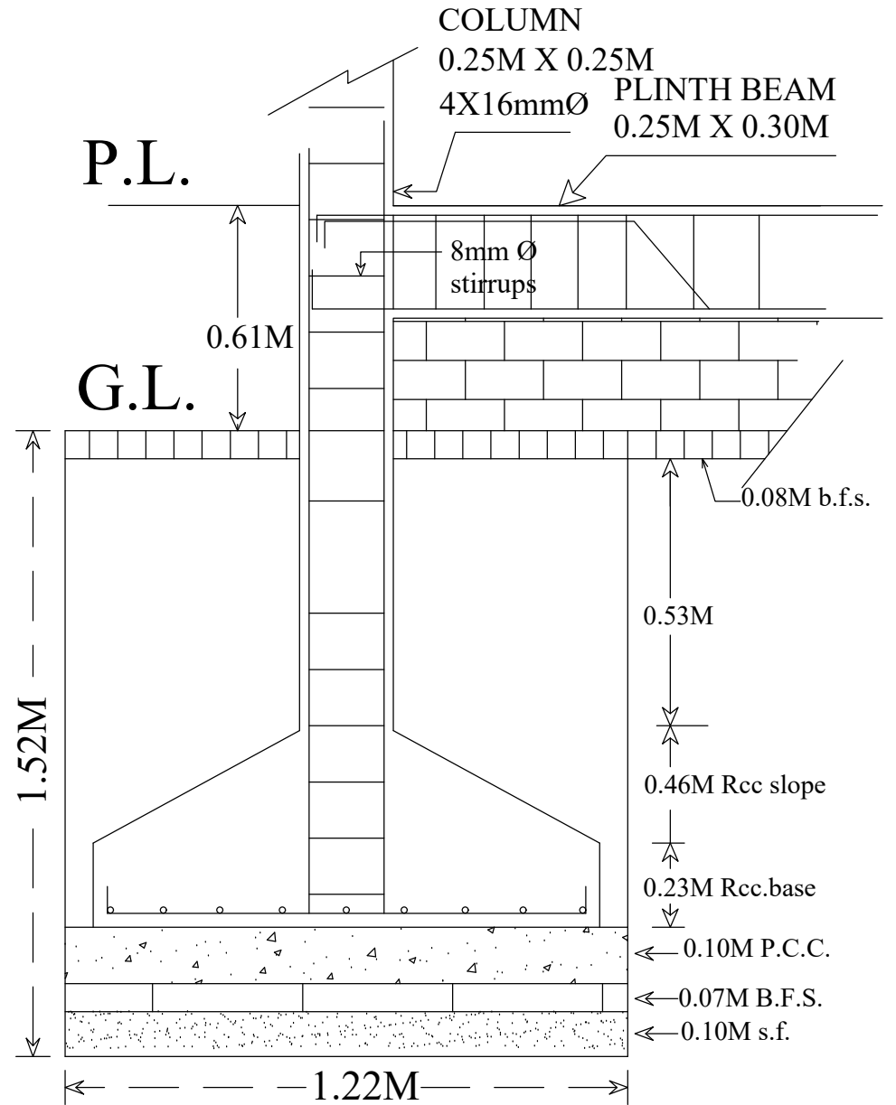
C/S OF FOOTING
