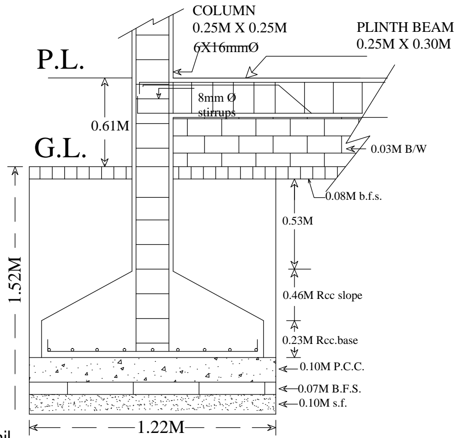
C/S OF FOOTING
