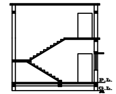
SECTION AT B-B
