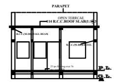
SECTION AT A-A
