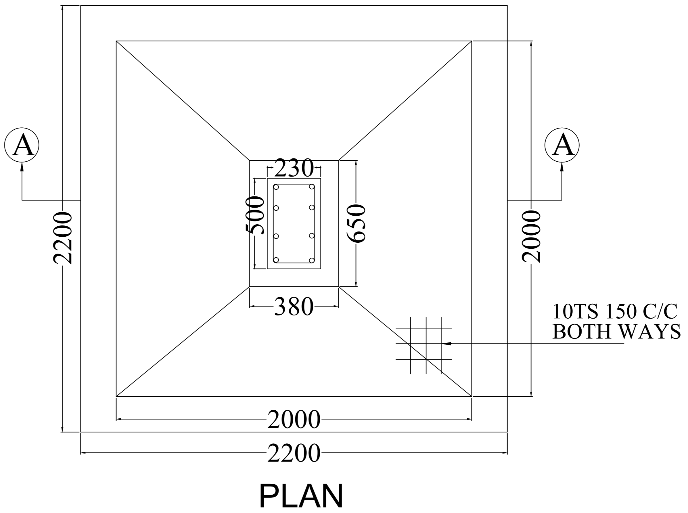
FOOTING PLAN (AS/STRL. DESIGN) SCALE N.T.S
