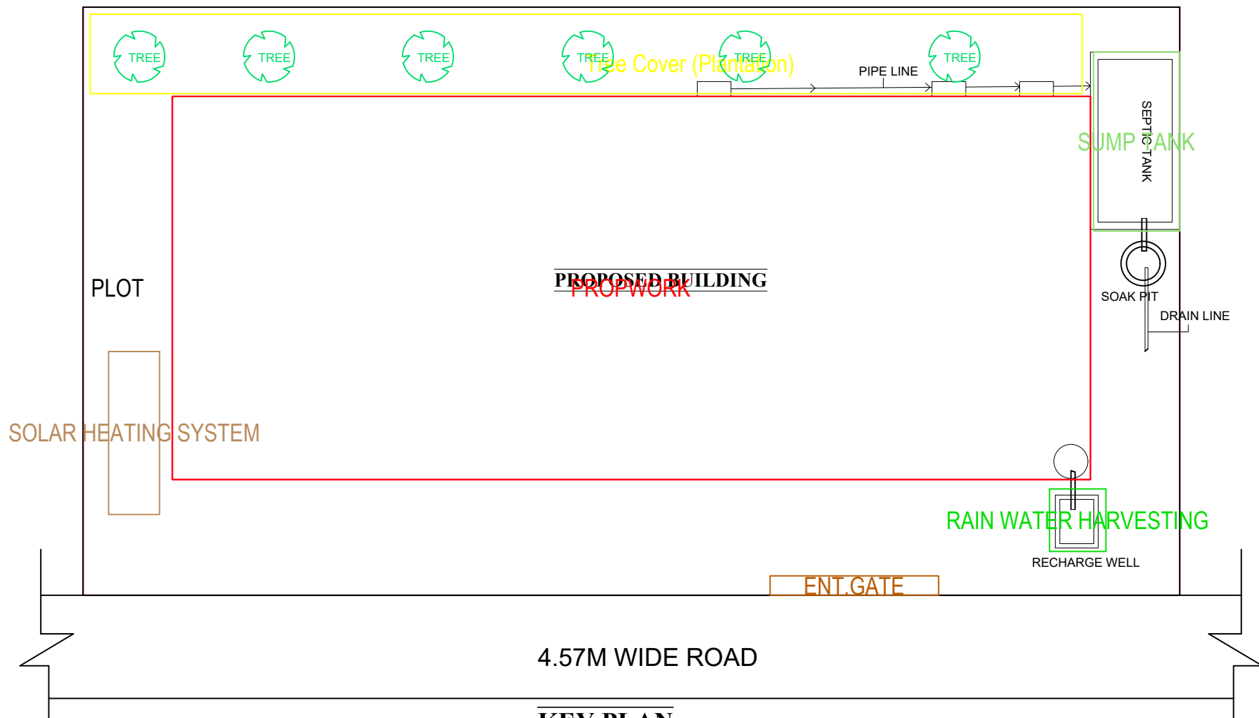
KEY PLAN EAST SIDE ROAD & FRONT SCALE-1:100
