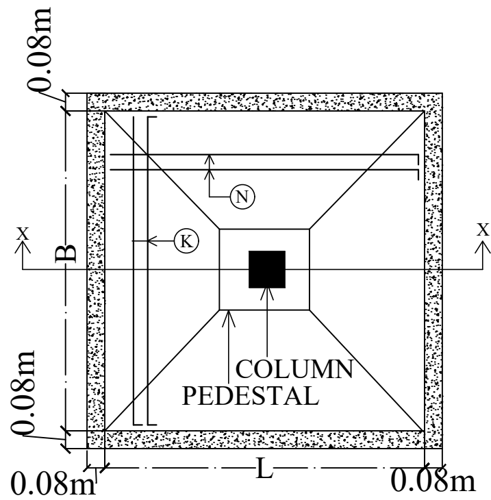
PLAN OF ISOLATED FOOTING
