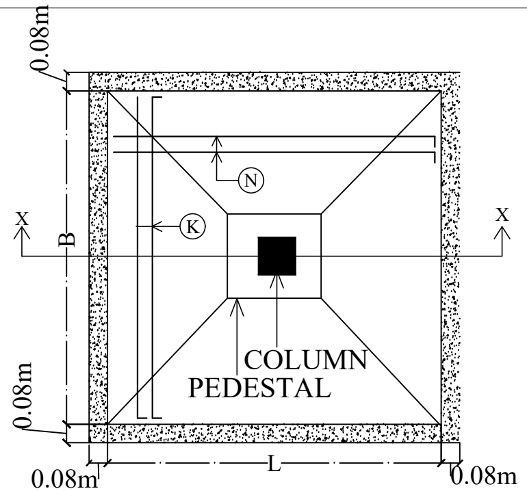
PLAN OF ISOLATED EX.FOOTING
