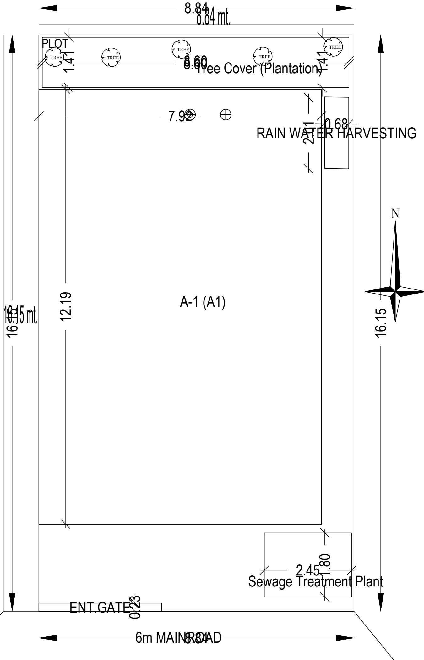
SITE PLAN
