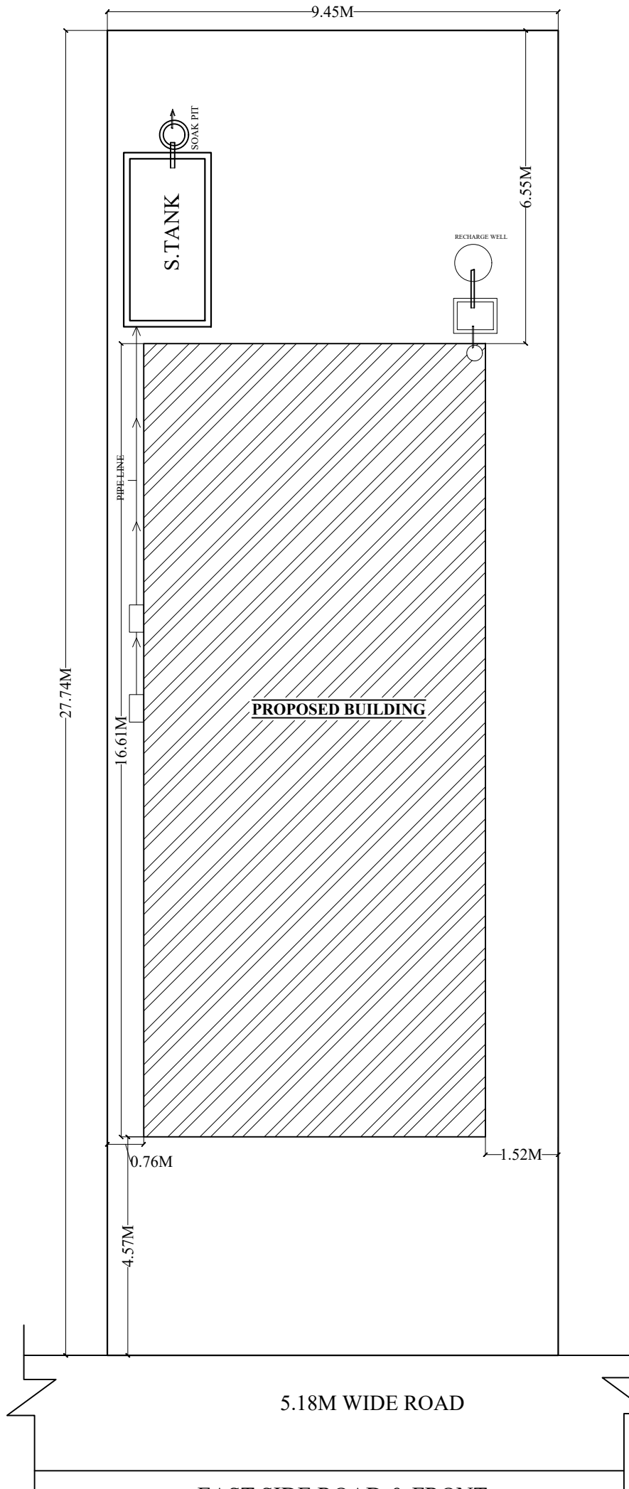
EAST SIDE ROAD & FRONT SCALE : 1:100 KEY PLAN
