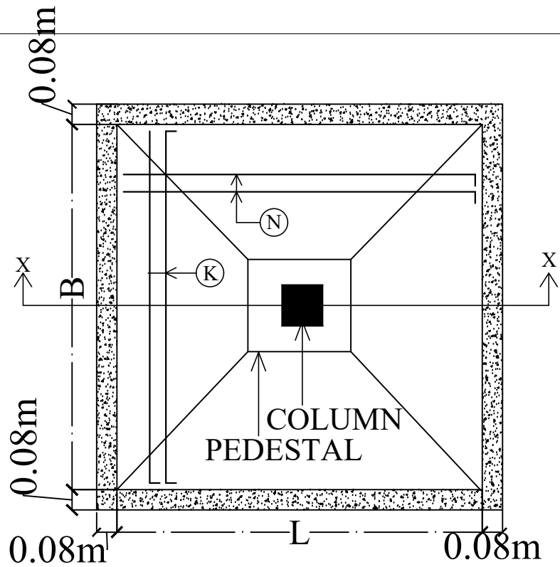
PLAN OF ISOLATED FOOTING
