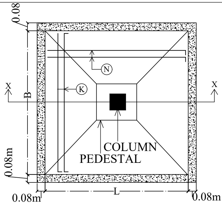
PLAN OF ISOLATED FOOTING
